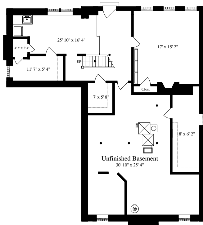
LOWER LEVEL
