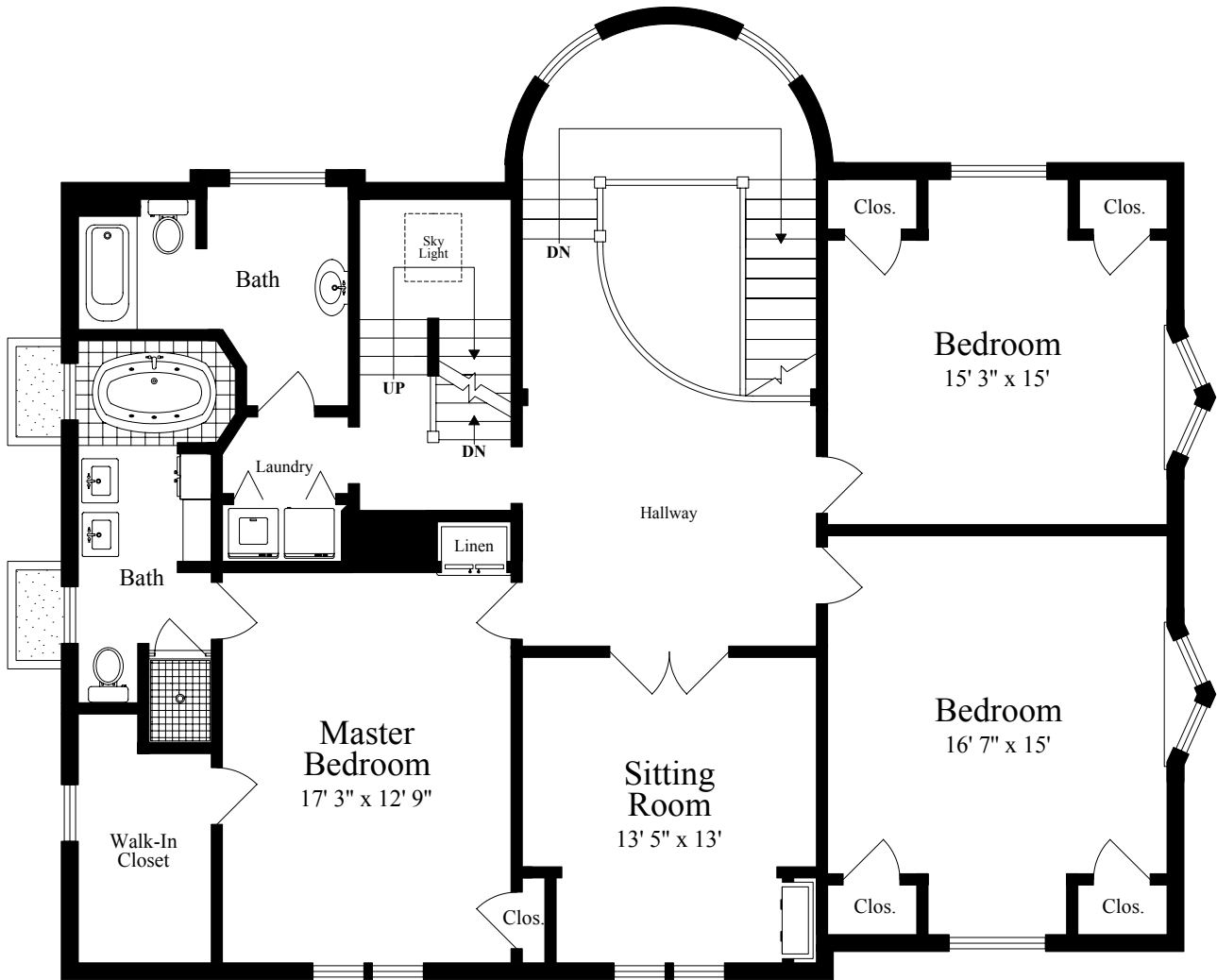
SECOND FLOOR
